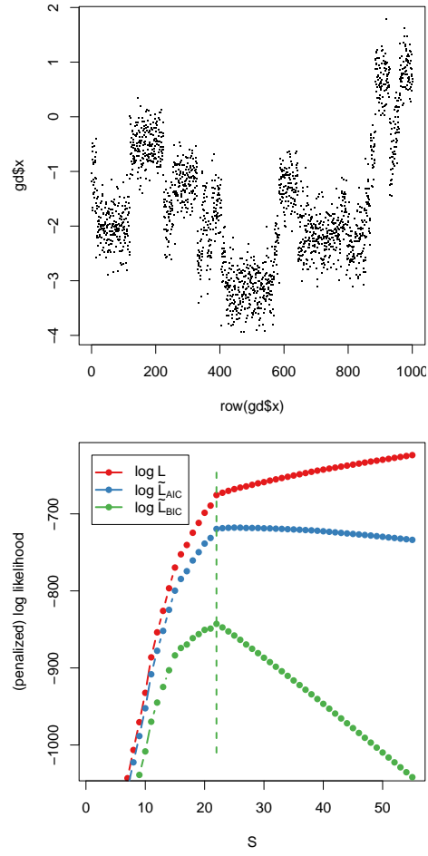
Figure 2: a) simulated data example with nrSeg=22 segments and vertical lines representing the fitted model with S=22 , selected by maximum \log L_{BIC} . b) log-likelihood \log L , penalized likelihoods \log \tilde{L}_{AIC} and \log \tilde{L}_{BIC} .
