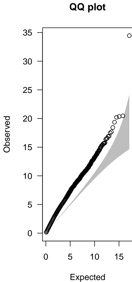
Expected distribution: chi-squared (1 df)
