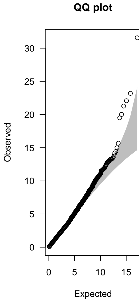
Expected distribution: chi-squared (1 df)
