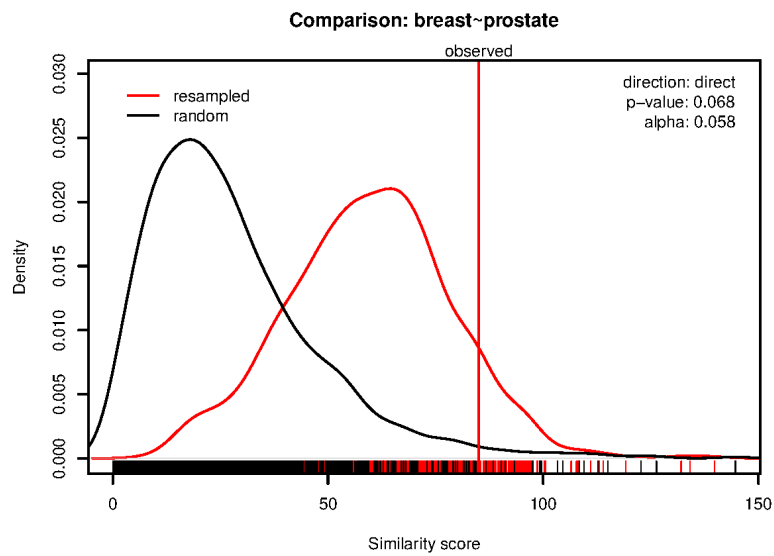
Figure 3.2: plot(x,"scores") : Shown are kernel density estimates of the two score distributions underlying the pAUC-score for optimal \alpha . The red curve corresponds to simulated observed scores and the black curve to simulated random scores. The vertical red line denotes the actually observed similarity score. The bottom rugs mark the simulated values. The two distributions got the highest pAUC-score of separability and thus provide the best signal-to-noise separation.
