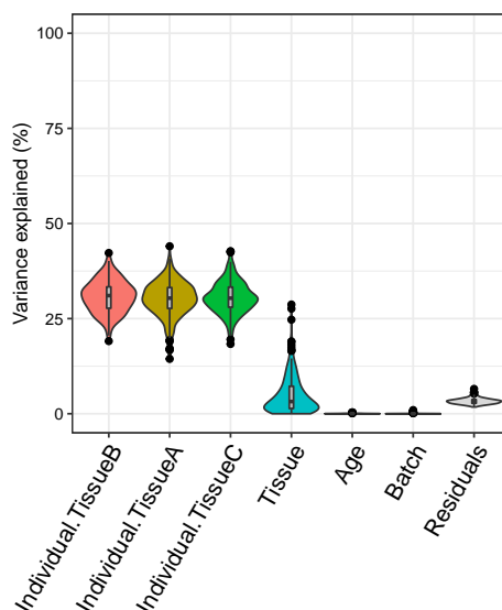
Figure 4: Variation across individuals within each tissue
