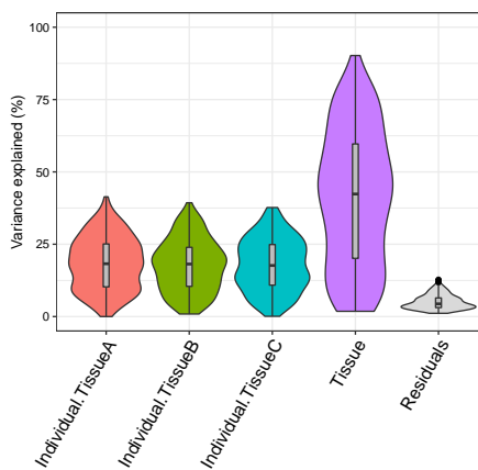
(f) variancePartition - within Tissue
