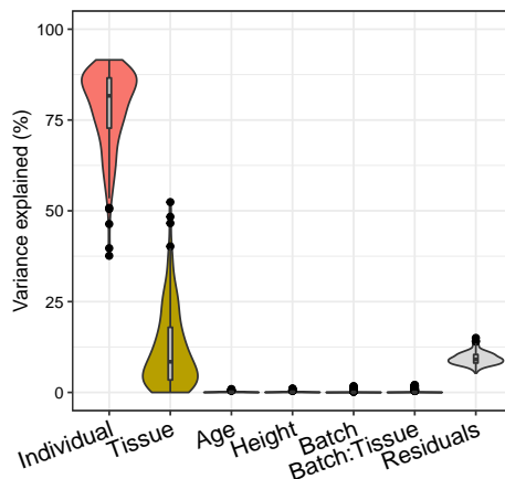
Figure 5: Fit interaction term
